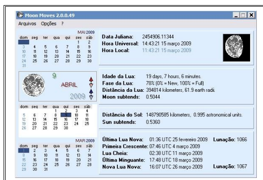
MoonMoves-2.0.0.exe
